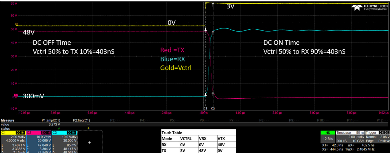
Figure 4. VCTRL to RX/TX Rise/Fall Time with SKY12248-492LF Connected: Vdd = 5 V, Vctrl 0/3V, RX/TX = 0/48 V (No RF): 2 uS/Div
