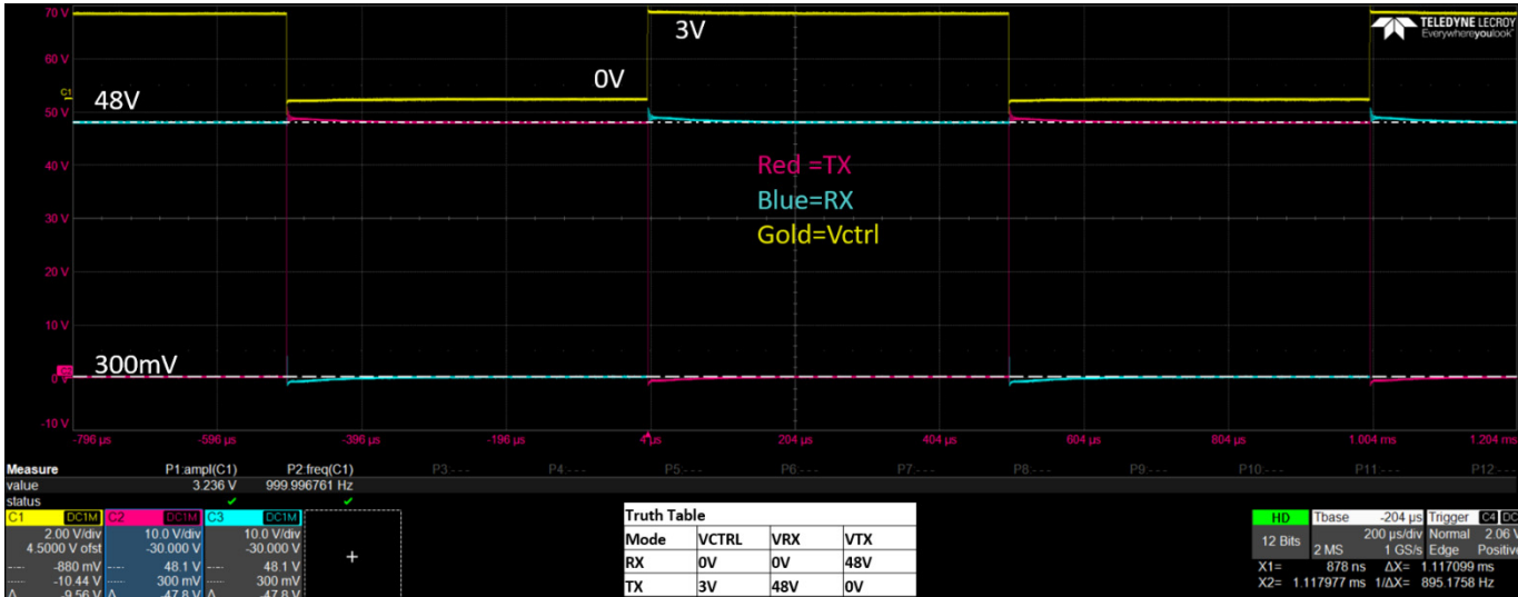
Figure 3. VCTRL to RX/TX Rise/Fall Time with SKY12248-492LF Connected: Vdd = 5 V, Vctrl 0/3V, RX/TX = 0/48 V (No RF): 200 uS/Div
