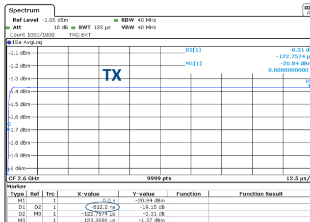
Figure 7. Skyworks High Power PIN Switch Evaluation Board + Driver Circuit RX Fall/TX Rise Time with HV Driver
